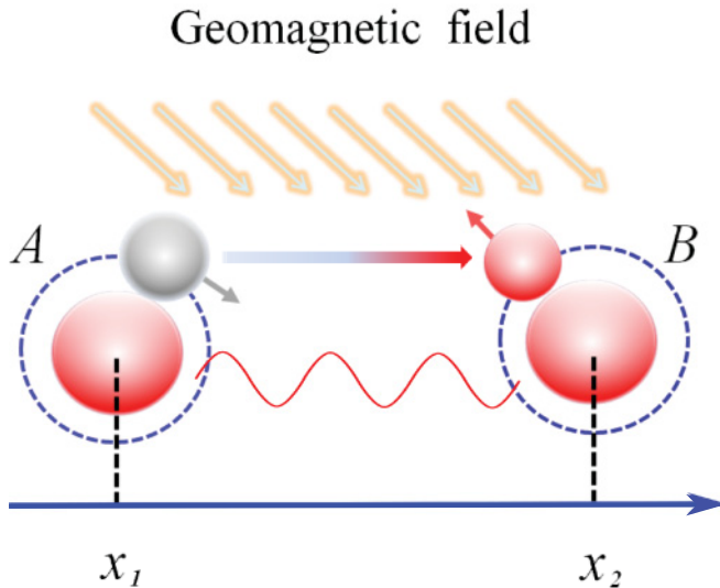
FIG. 1. (Color online) Schematic of the generalized Holstein model. It is composed of a radical pair with nuclear spins. Two electrons are initially prepared in a correlated state (i.e., the singlet state or triplet state), which can be interconverted by the hyperfine interaction in combination with an external magnetic field. The chemical reaction occurs once both electrons are in the same site due to the tunneling effect.
