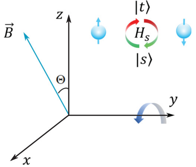
FIG. 2. (Color online) The inclination angle between the external geomagnetic field and the z direction is \Theta , and the coordinate system is rotated around the y axis with \Theta to coincide with the direction of the magnetic field. The hyperfine-coupling-induced interconversion between the singlet and triplet states is modulated by the direction of the magnetic field (i.e., \Theta ).
