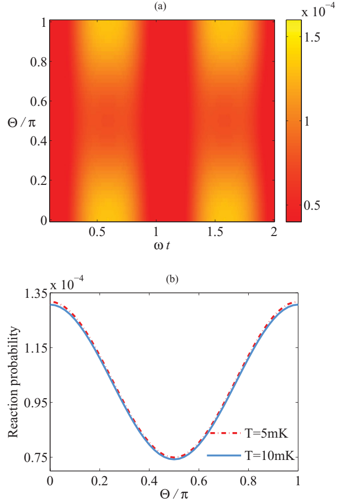
FIG. 3. (Color online) (a) Chemical reaction probability vs time and \Theta . (b) Chemical reaction probability for triplet state at a given time t = 0.5/\omega for effective temperature T = 5 mK (red dashed line) and T = 10 mK (blue solid line).
