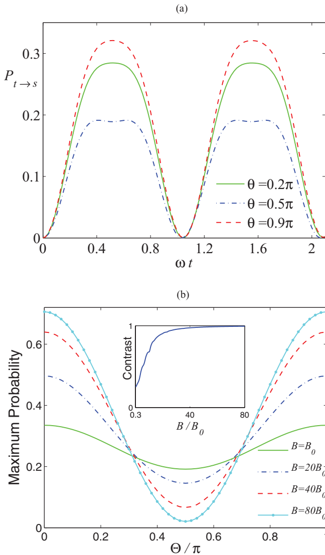
FIG. 4. (Color online) Transition probability from triplet state to singlet state. (a) Probability vs time for different angles. (b) The maximum probability varies with angle for the applied field with different magnitudes. The inset shows that the contrast of the maximum transition probability also changes with the magnitude of the magnetic field.
